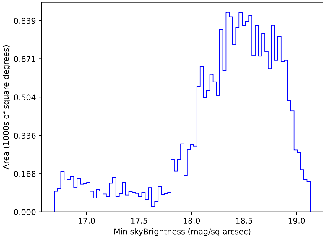
too_elab_r32_d3_ugrizy_v3.4_10yrs Yr 1 z band: Min skyBrightness
