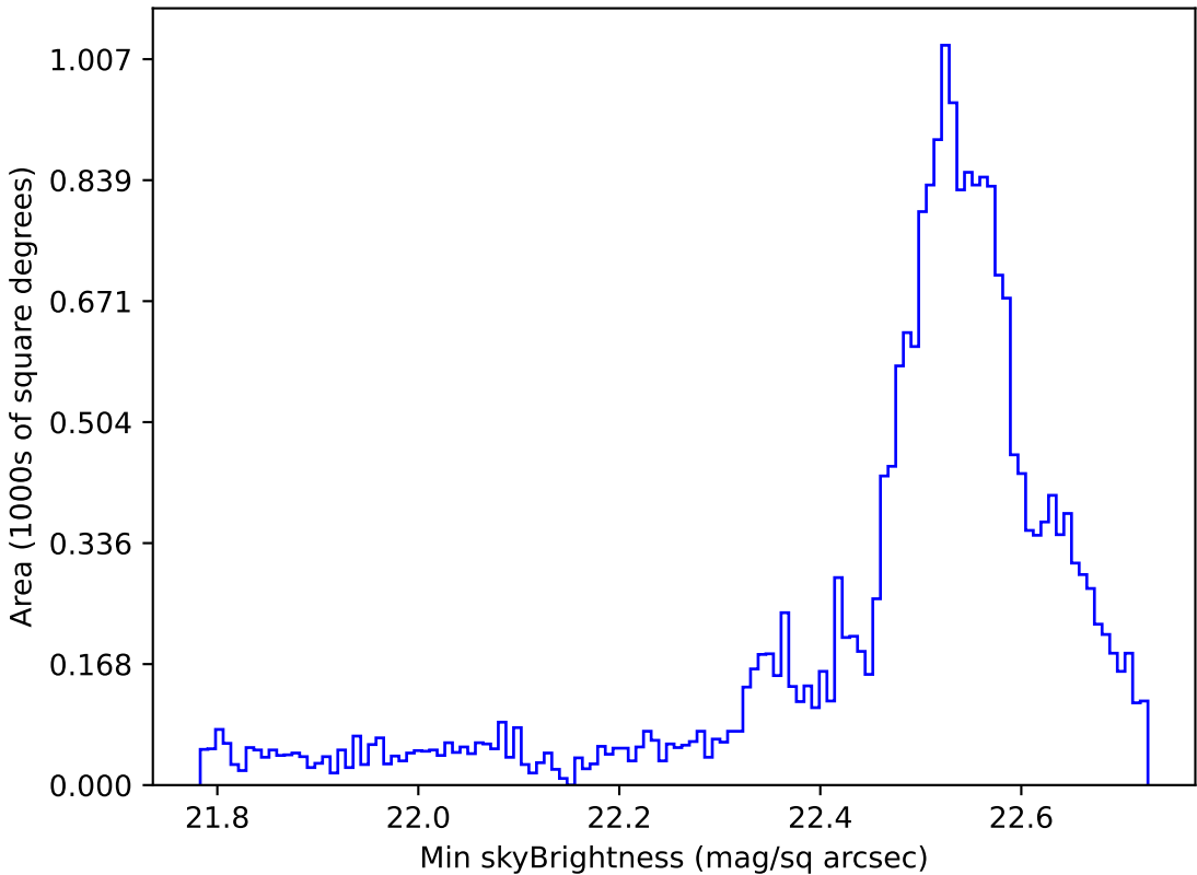
too_elab_r32_d3_ugrizy_v3.4_10yrs Yr 1 u band: Min skyBrightness
