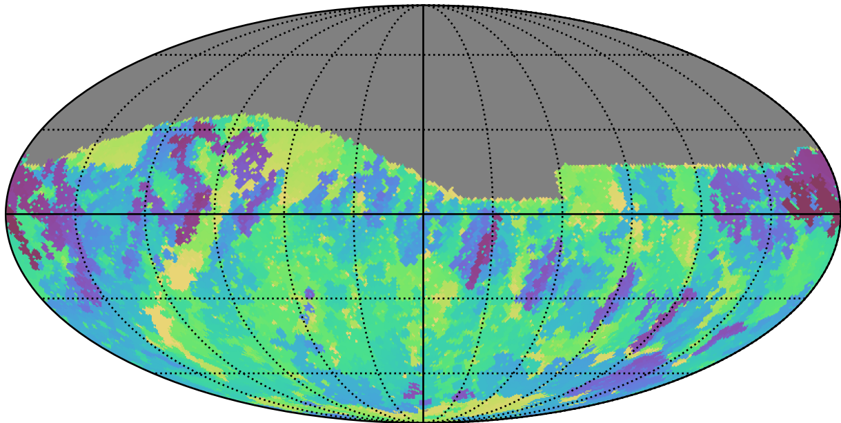
too_elab_r32_d3_ugrizy_v3.4_10yrs Yr 1 r band: Min skyBrightness
