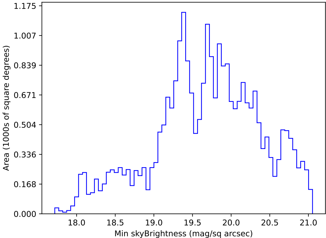
too_elab_r32_d3_ugrizy_v3.4_10yrs Yr 1 r band: Min skyBrightness
