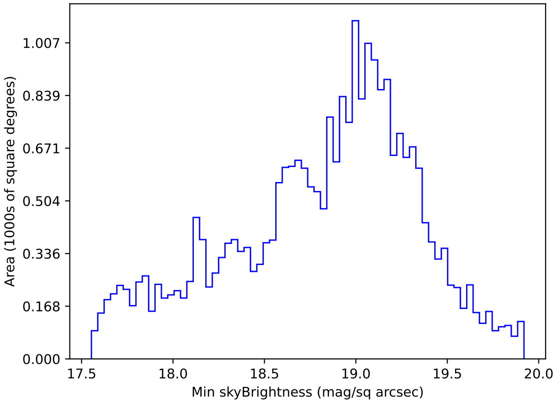
too_elab_r32_d3_ugrizy_v3.4_10yrs Yr 1 i band: Min skyBrightness
