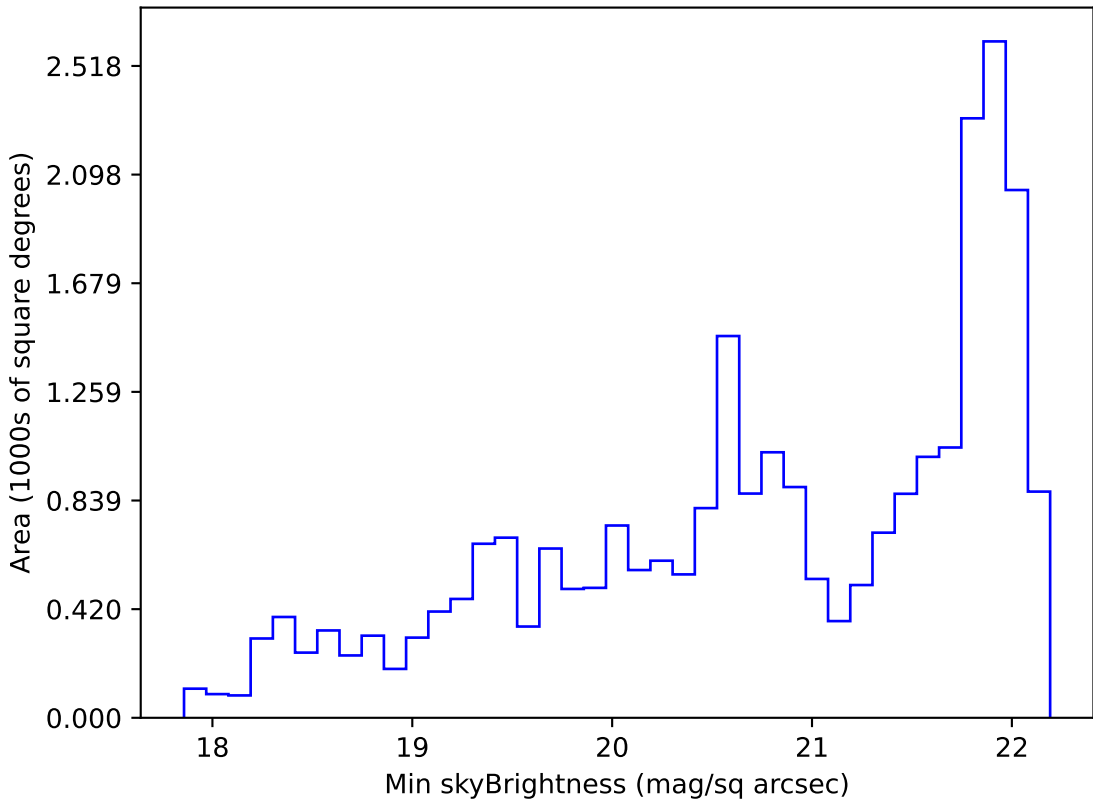
too_elab_r32_d3_ugrizy_v3.4_10yrs Yr 1 g band: Min skyBrightness
