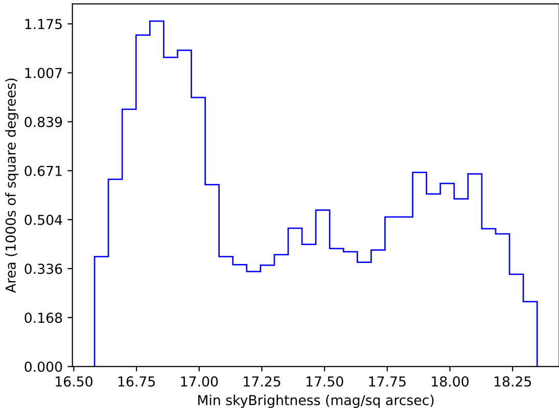
too_elab_r32_d3_ugrizy_v3.4_10yrs WFD z band: Min skyBrightness
