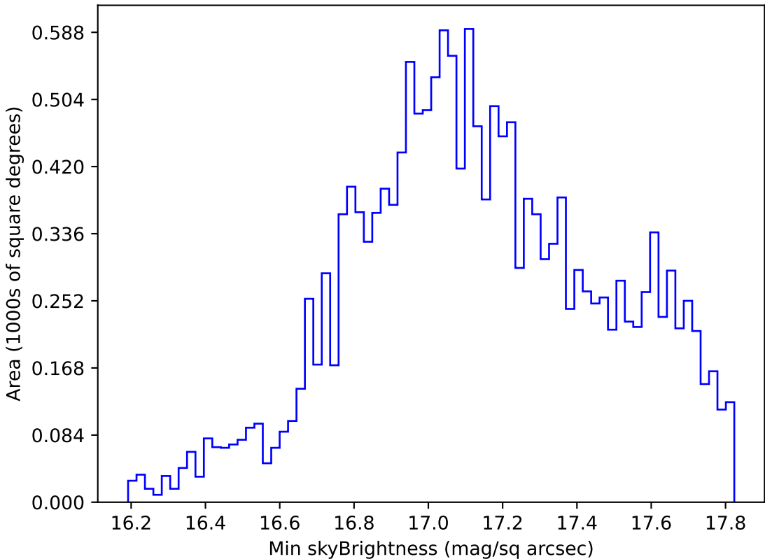
too_elab_r32_d3_ugrizy_v3.4_10yrs WFD y band: Min skyBrightness
