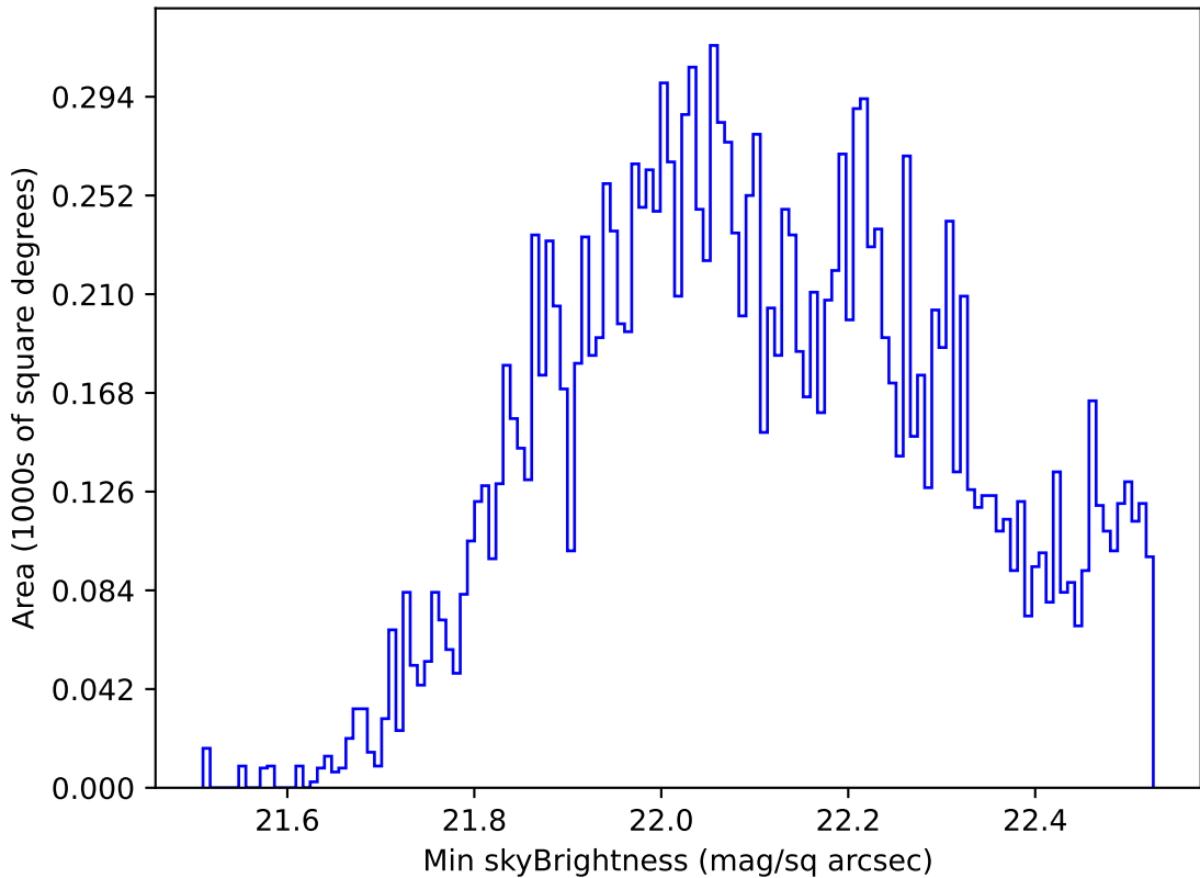
too_elab_r32_d3_ugrizy_v3.4_10yrs WFD u band: Min skyBrightness
