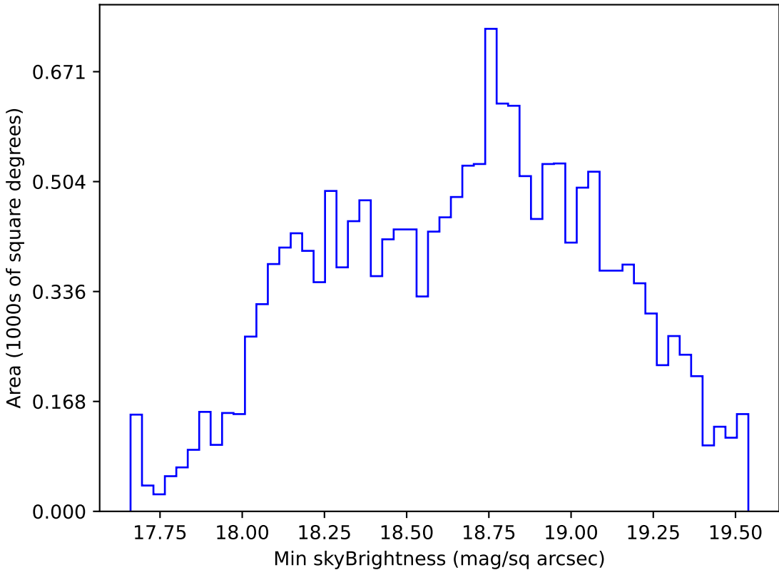
too_elab_r32_d3_ugrizy_v3.4_10yrs WFD r band: Min skyBrightness
