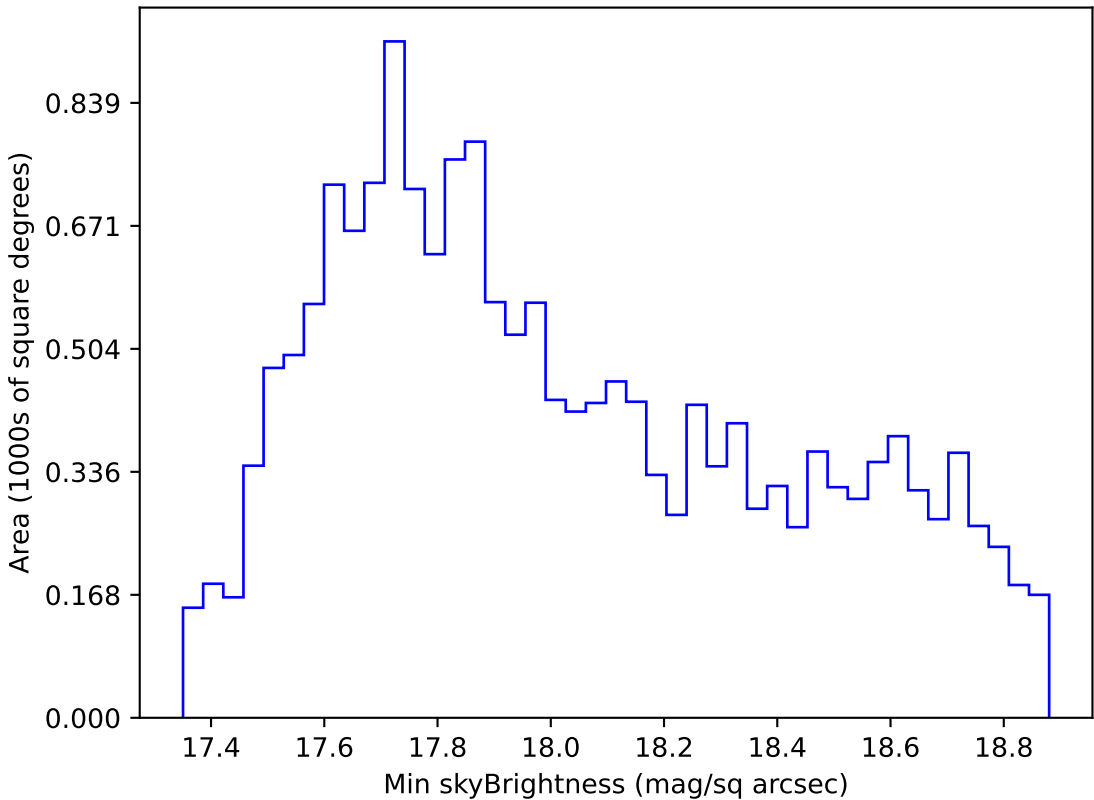
too_elab_r32_d3_ugrizy_v3.4_10yrs WFD i band: Min skyBrightness
