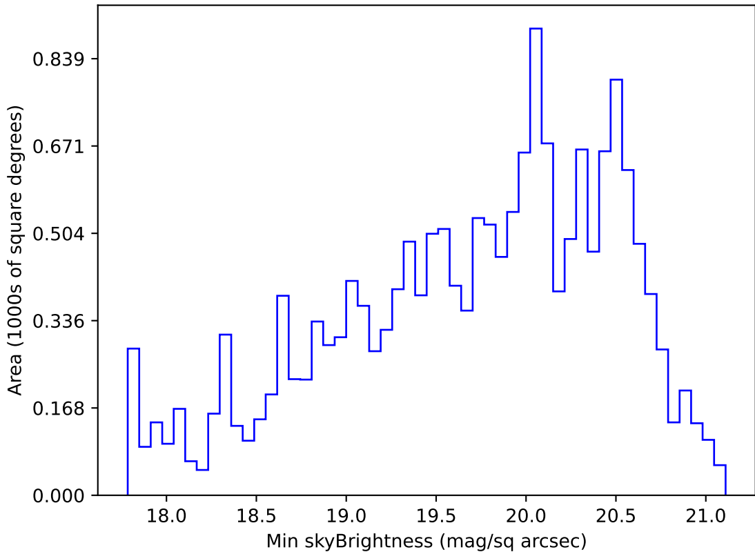
too_elab_r32_d3_ugrizy_v3.4_10yrs WFD g band: Min skyBrightness
