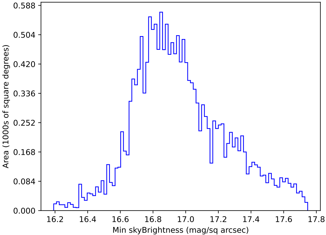
too_elab_r32_d3_ugrizy_v3.4_10yrs WFD all bands: Min skyBrightness
