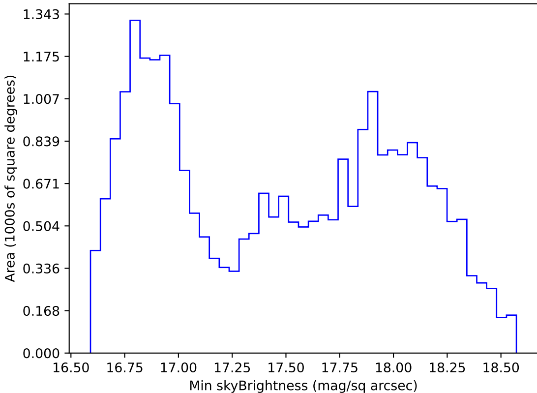
too_elab_r32_d3_ugrizy_v3.4_10yrs All sky z band: Min skyBrightness
