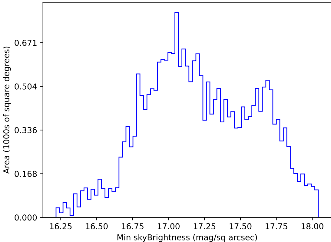
too_elab_r32_d3_ugrizy_v3.4_10yrs All sky y band: Min skyBrightness
