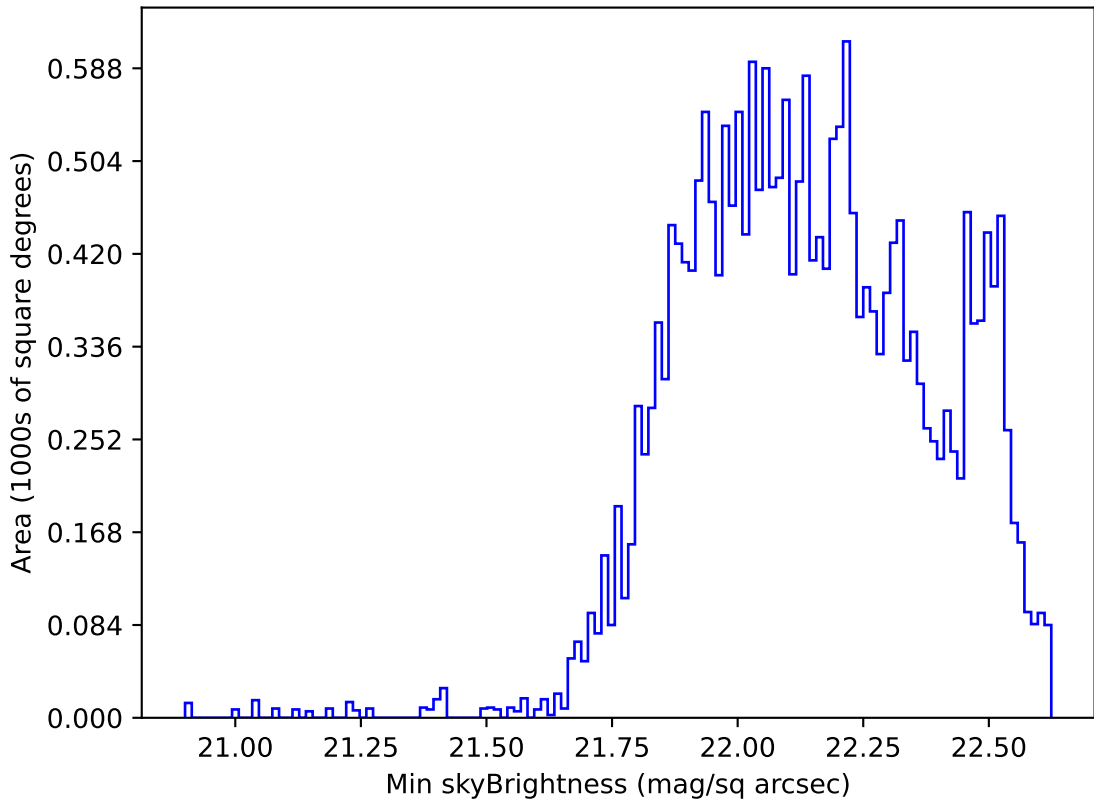
too_elab_r32_d3_ugrizy_v3.4_10yrs All sky u band: Min skyBrightness
