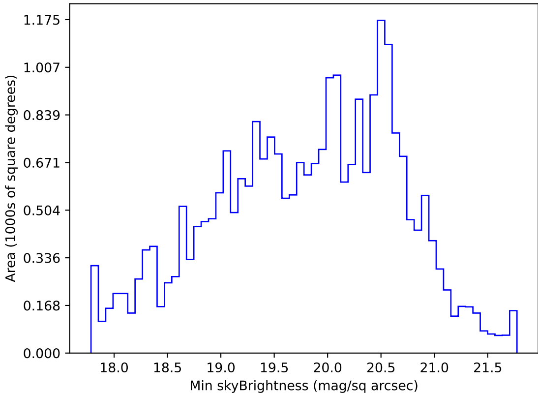
too_elab_r32_d3_ugrizy_v3.4_10yrs All sky g band: Min skyBrightness
