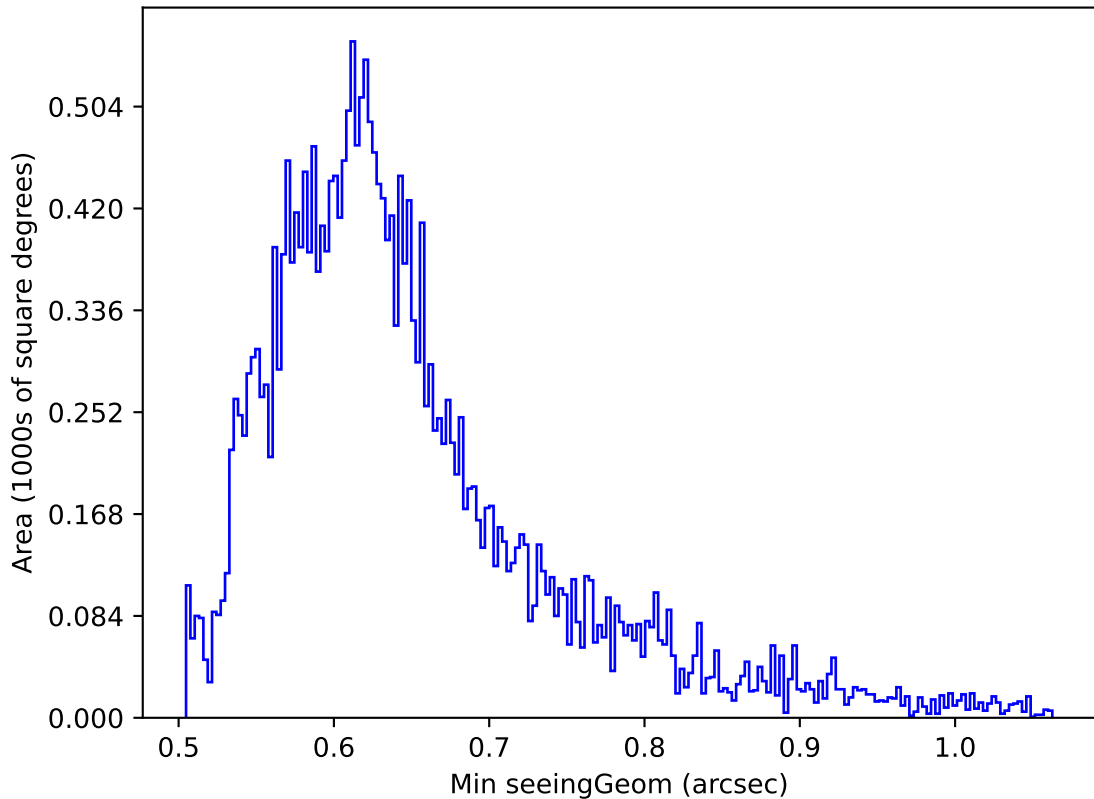
too_elab_r32_d3_ugrizy_v3.4_10yrs Yr 1 z band: Min seeingGeom
