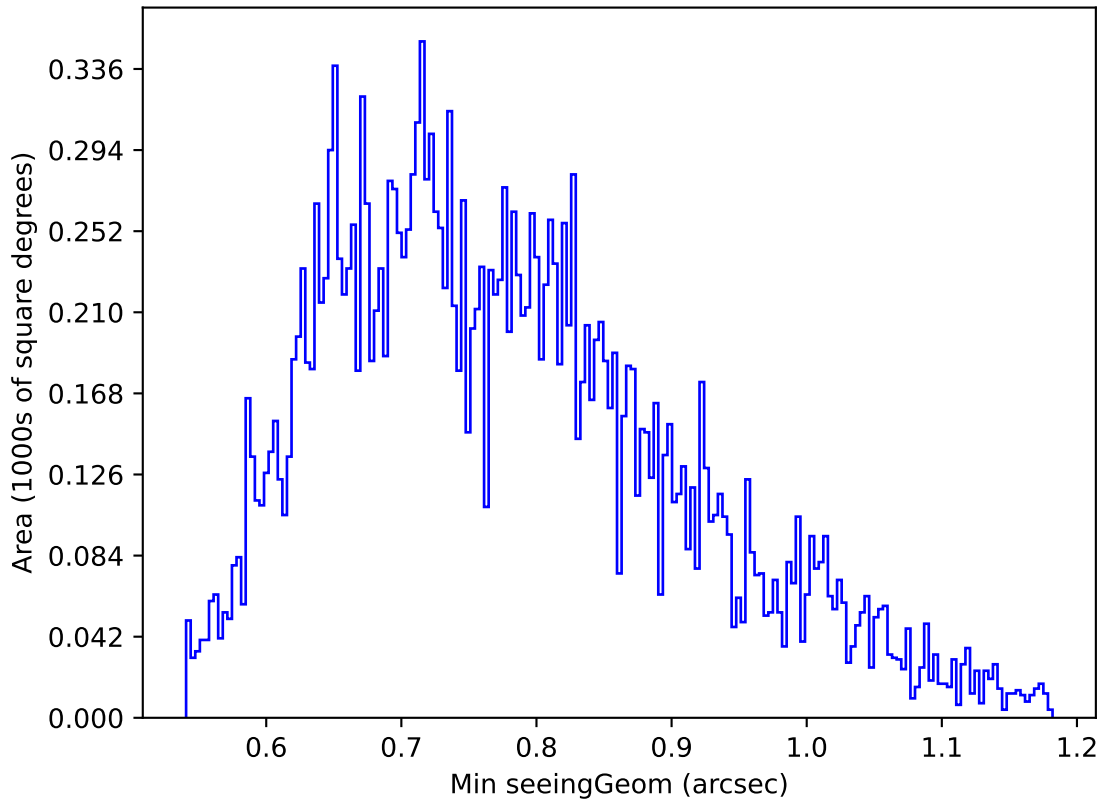
too_elab_r32_d3_ugrizy_v3.4_10yrs Yr 1 u band: Min seeingGeom
