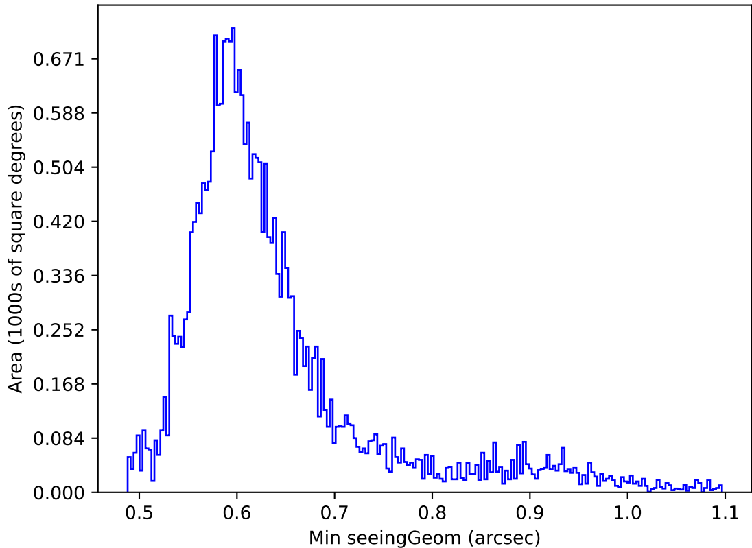
too_elab_r32_d3_ugrizy_v3.4_10yrs Yr 1 i band: Min seeingGeom
