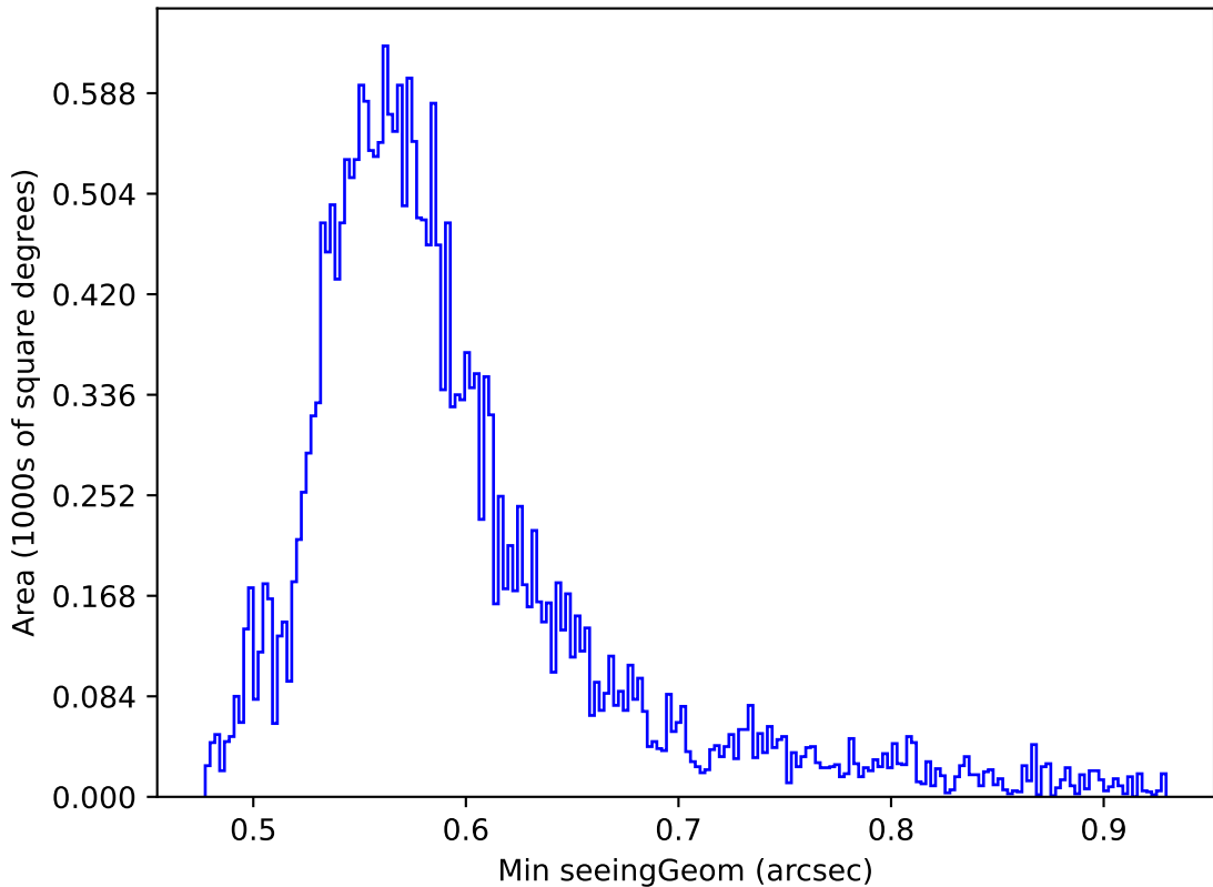
too_elab_r32_d3_ugrizy_v3.4_10yrs Yr 1 all bands: Min seeingGeom
