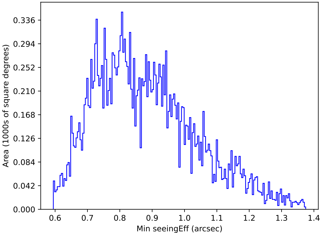
too_elab_r32_d3_ugrizy_v3.4_10yrs Yr 1 u band: Min seeingEff
