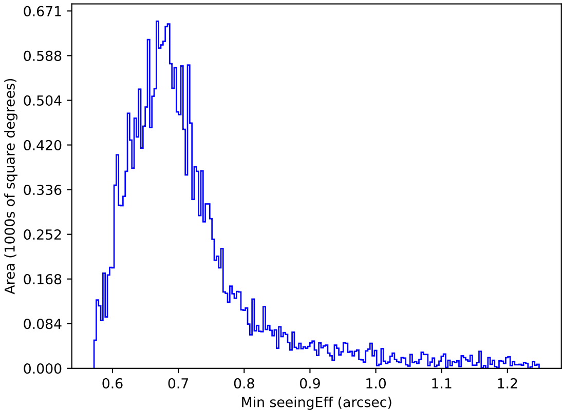
too_elab_r32_d3_ugrizy_v3.4_10yrs Yr 1 r band: Min seeingEff
