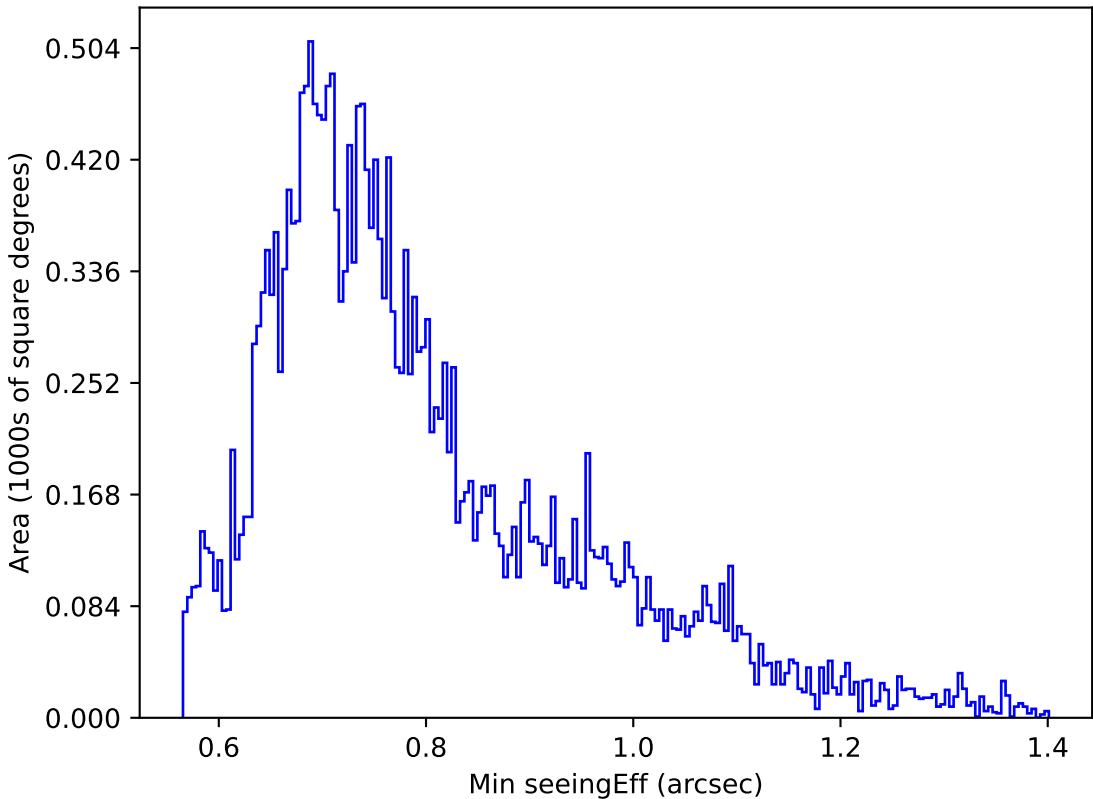
too_elab_r32_d3_ugrizy_v3.4_10yrs Yr 1 g band: Min seeingEff
