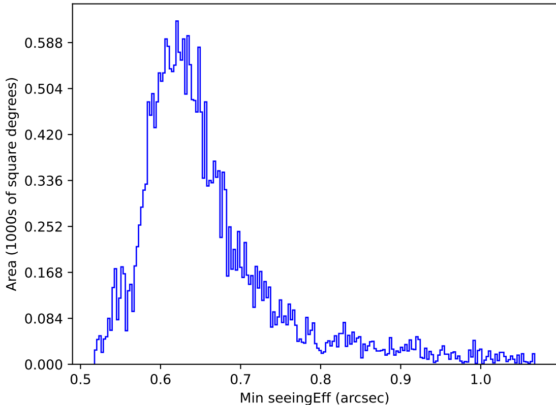
too_elab_r32_d3_ugrizy_v3.4_10yrs Yr 1 all bands: Min seeingEff
