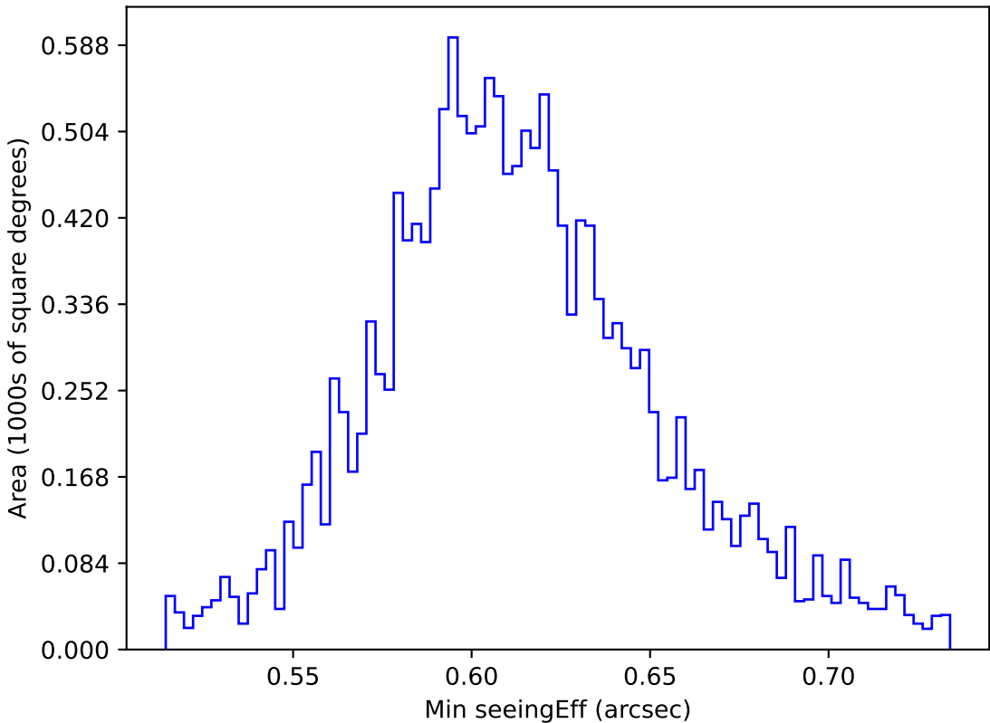
too_elab_r32_d3_ugrizy_v3.4_10yrs WFD z band: Min seeingEff
