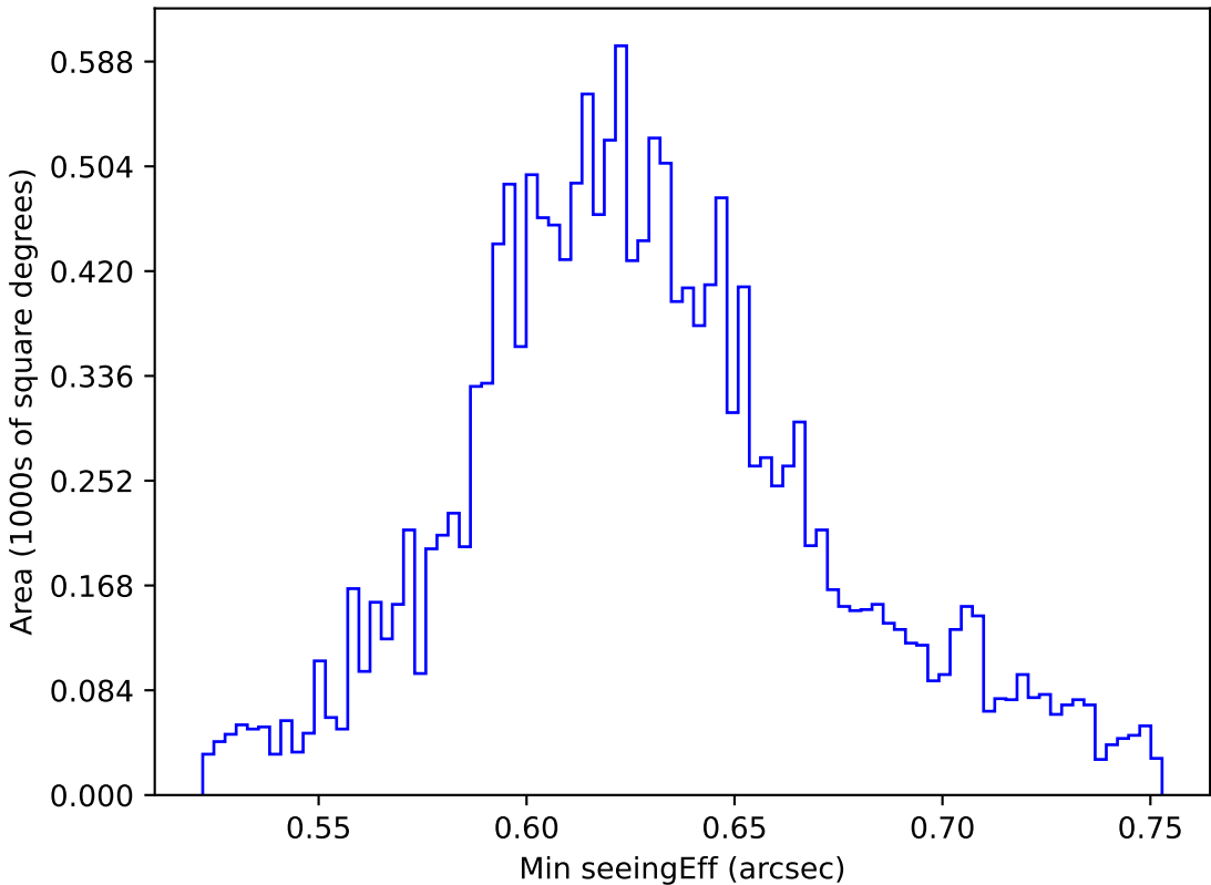
too_elab_r32_d3_ugrizy_v3.4_10yrs WFD y band: Min seeingEff
