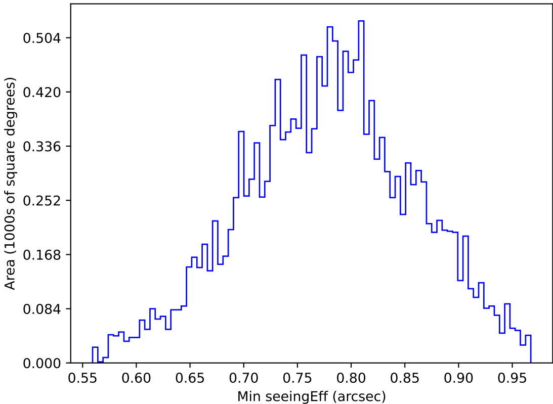
too_elab_r32_d3_ugrizy_v3.4_10yrs WFD u band: Min seeingEff
