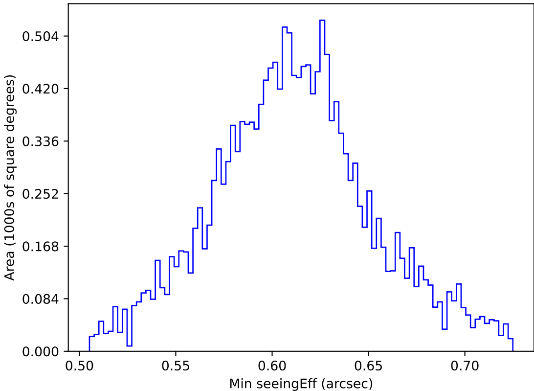
too_elab_r32_d3_ugrizy_v3.4_10yrs WFD r band: Min seeingEff
