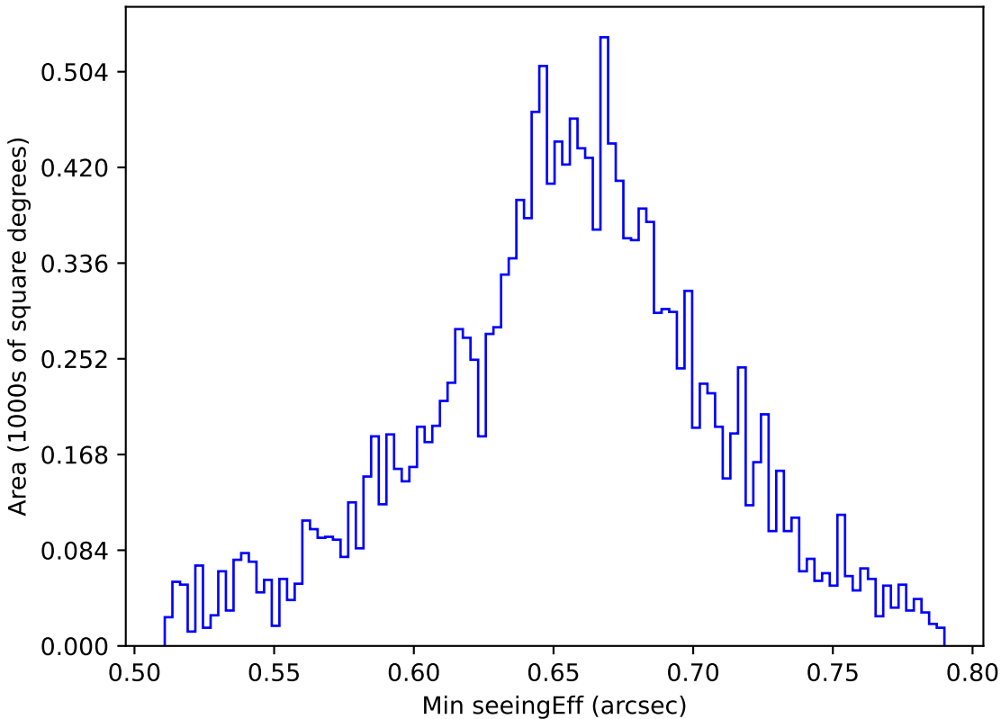
too_elab_r32_d3_ugrizy_v3.4_10yrs WFD g band: Min seeingEff
