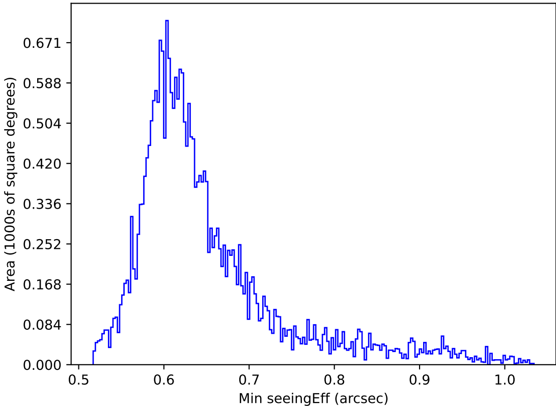
too_elab_r32_d3_ugrizy_v3.4_10yrs All sky z band: Min seeingEff
