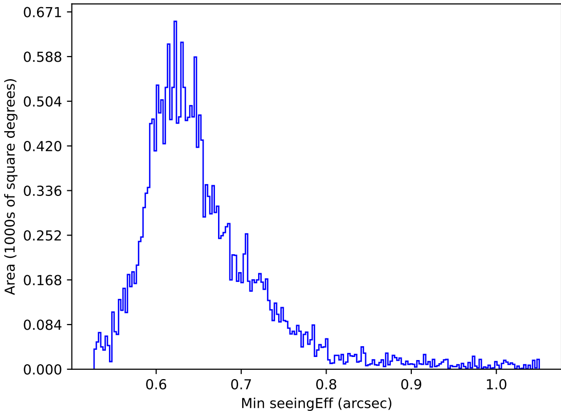
too_elab_r32_d3_ugrizy_v3.4_10yrs All sky y band: Min seeingEff
