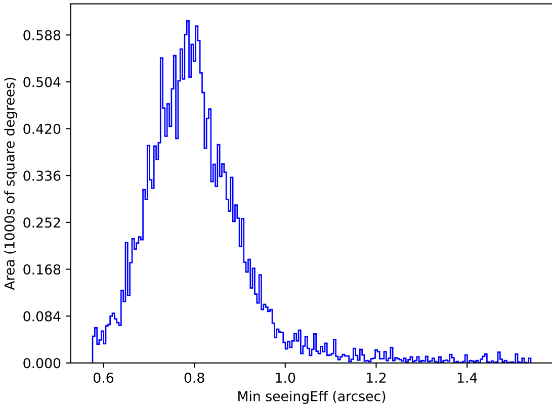
too_elab_r32_d3_ugrizy_v3.4_10yrs All sky u band: Min seeingEff
