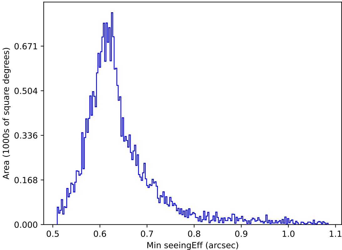
too_elab_r32_d3_ugrizy_v3.4_10yrs All sky r band: Min seeingEff
