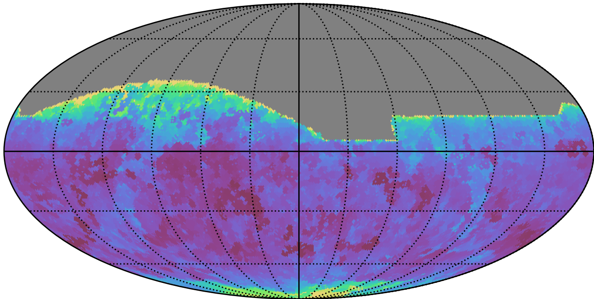
too_elab_r32_d3_ugrizy_v3.4_10yrs All sky i band: Min seeingEff
