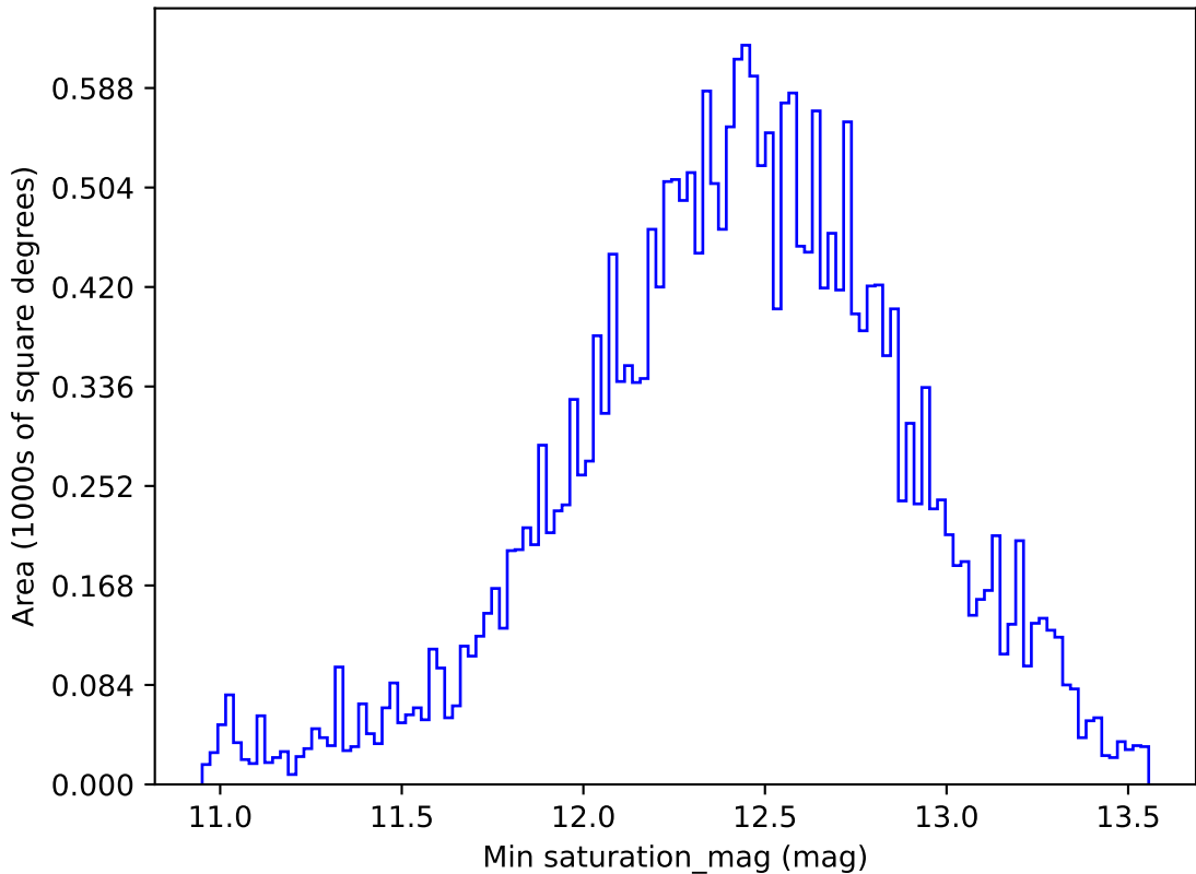
too_elab_r32_d3_ugrizy_v3.4_10yrs All sky i band: Min saturation_mag
