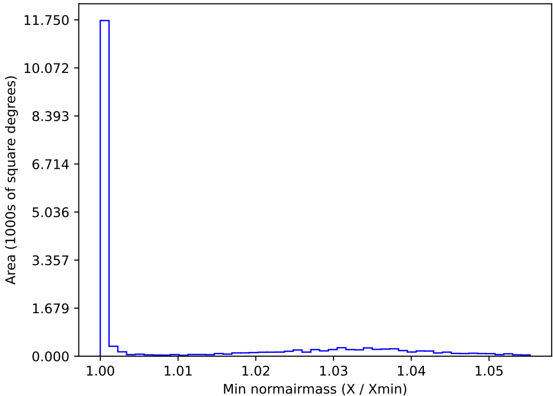
too_elab_r32_d3_ugrizy_v3.4_10yrs WFD u band: Min normairmass
