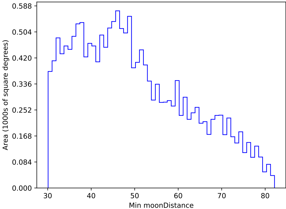
too_elab_r32_d3_ugrizy_v3.4_10yrs WFD u band: Min moonDistance
