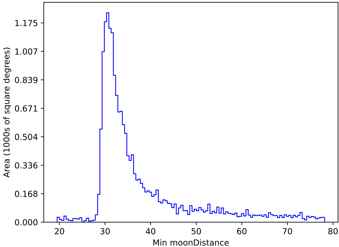
too_elab_r32_d3_ugrizy_v3.4_10yrs WFD r band: Min moonDistance
