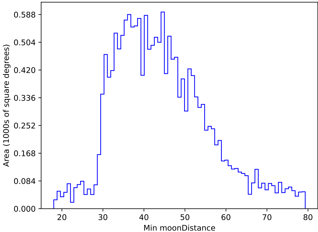
too_elab_r32_d3_ugrizy_v3.4_10yrs WFD g band: Min moonDistance
