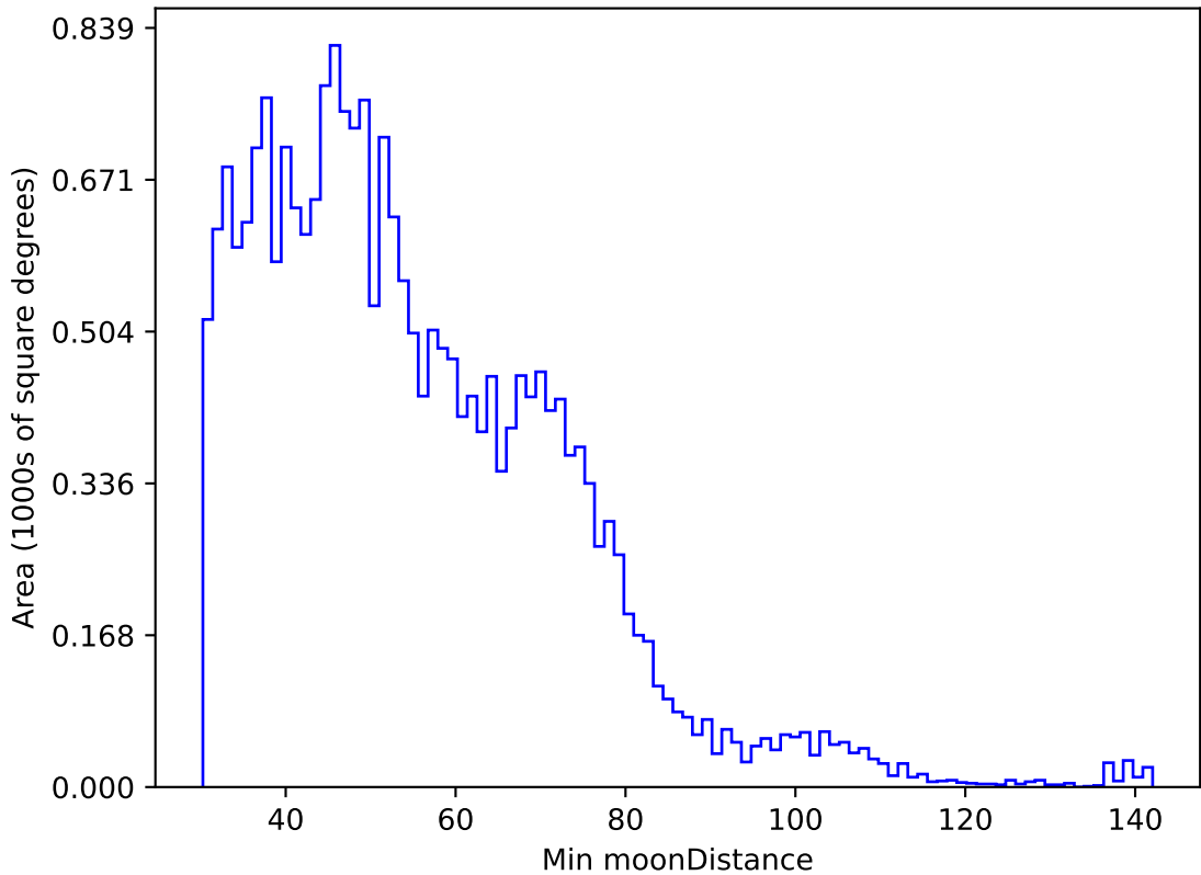
too_elab_r32_d3_ugrizy_v3.4_10yrs All sky u band: Min moonDistance
