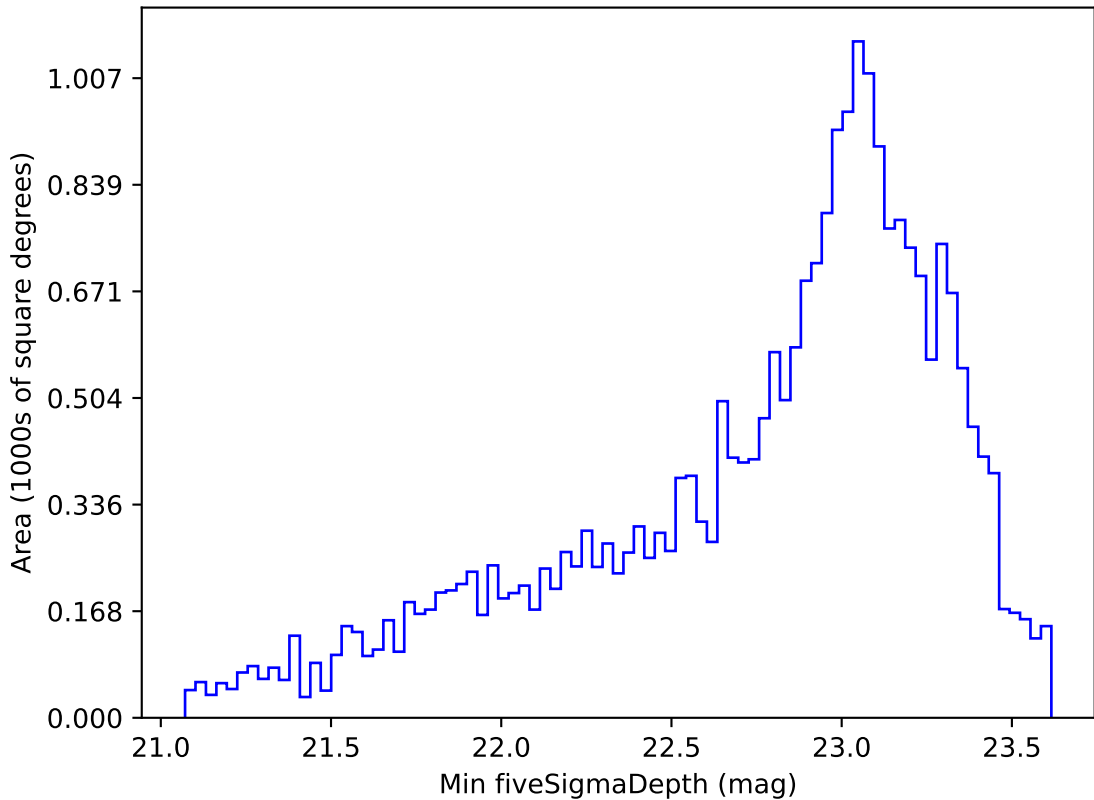
too_elab_r32_d3_ugrizy_v3.4_10yrs Yr 1 i band: Min fiveSigmaDepth
