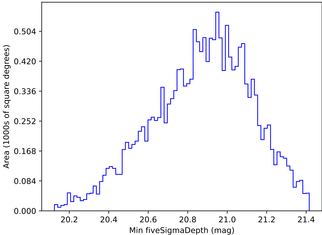
too_elab_r32_d3_ugrizy_v3.4_10yrs WFD y band: Min fiveSigmaDepth
