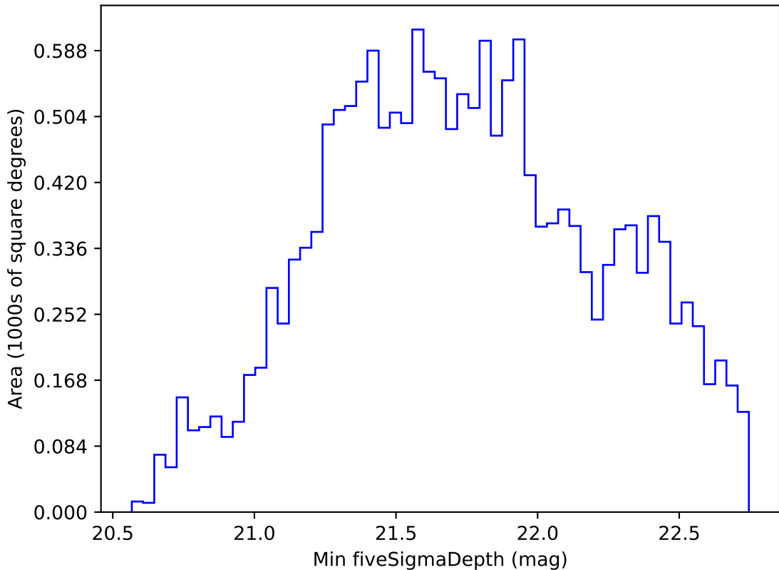
too_elab_r32_d3_ugrizy_v3.4_10yrs WFD i band: Min fiveSigmaDepth
