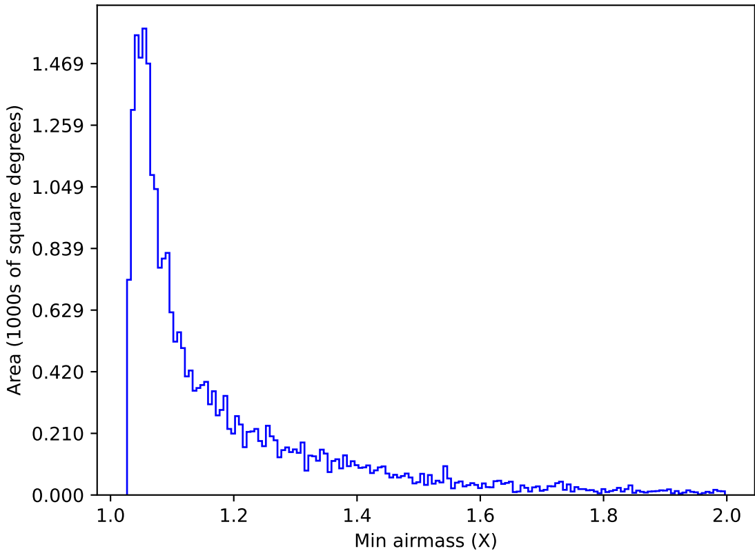
too_elab_r32_d3_ugrizy_v3.4_10yrs Yr 1 g band: Min airmass
