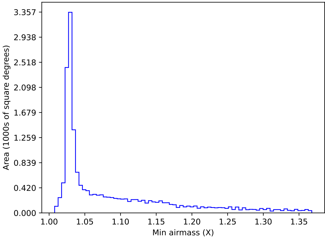
too_elab_r32_d3_ugrizy_v3.4_10yrs WFD z band: Min airmass
