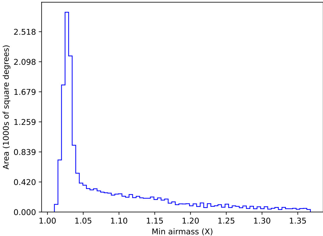
too_elab_r32_d3_ugrizy_v3.4_10yrs WFD r band: Min airmass
