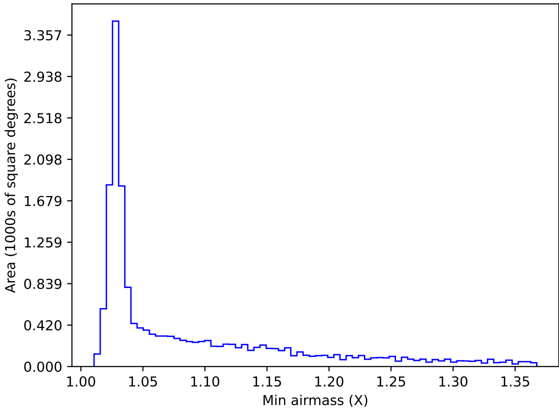
too_elab_r32_d3_ugrizy_v3.4_10yrs WFD i band: Min airmass
