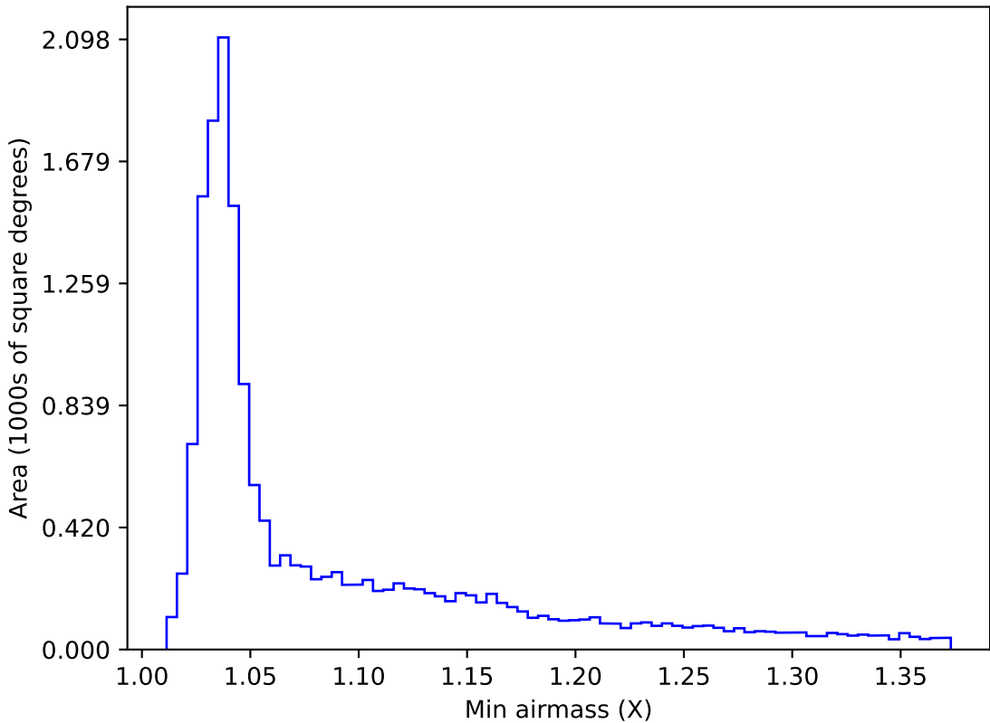
too_elab_r32_d3_ugrizy_v3.4_10yrs WFD g band: Min airmass
