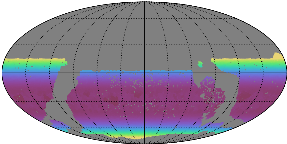
too_elab_r32_d3_ugrizy_v3.4_10yrs WFD all bands: Min airmass
